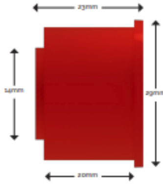
CAPILLARY ADAPTOR
