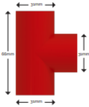
TEE ADAPTOR
