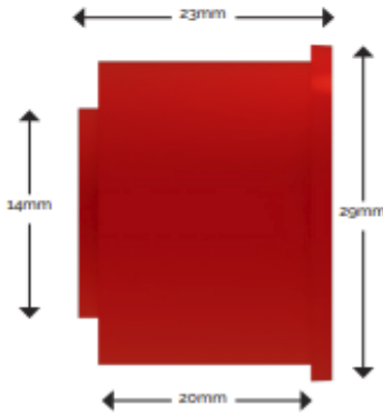
CAPILLARY ADAPTOR
