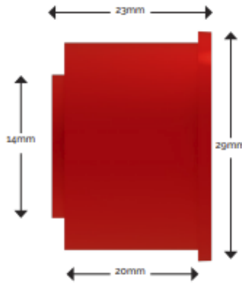
CAPILLARY ADAPTOR
