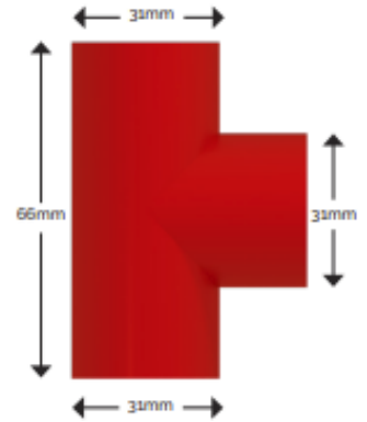
TEE FRONT ELEVATION
